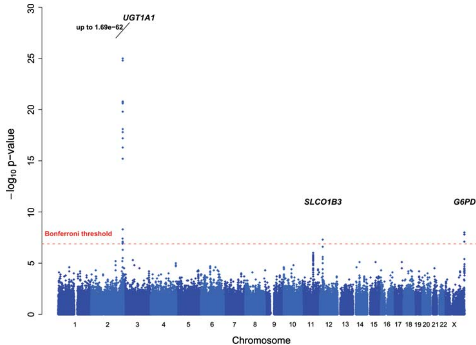
Figure 1. Genome-wide scan of serum total bilirubin. The figure summarizes association P -values (additive test) for all SNPs that passed quality control tests ( N = 362,129 ). Position of UGT1A1 , SLCO1B3 and G6PD genes are annotated. Red dotted line marks Bonferroni threshold ( 1.3 \times 10^{-7} ).
