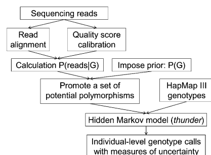
Figure 4. Genotype calling pipeline for the 1000 Genomes Pilot 1 Project. The pipeline we have developed to call genotypes for individuals sequenced at an average depth of \sim 4–5\times by the 1000 Genomes Pilot 1 Project.
