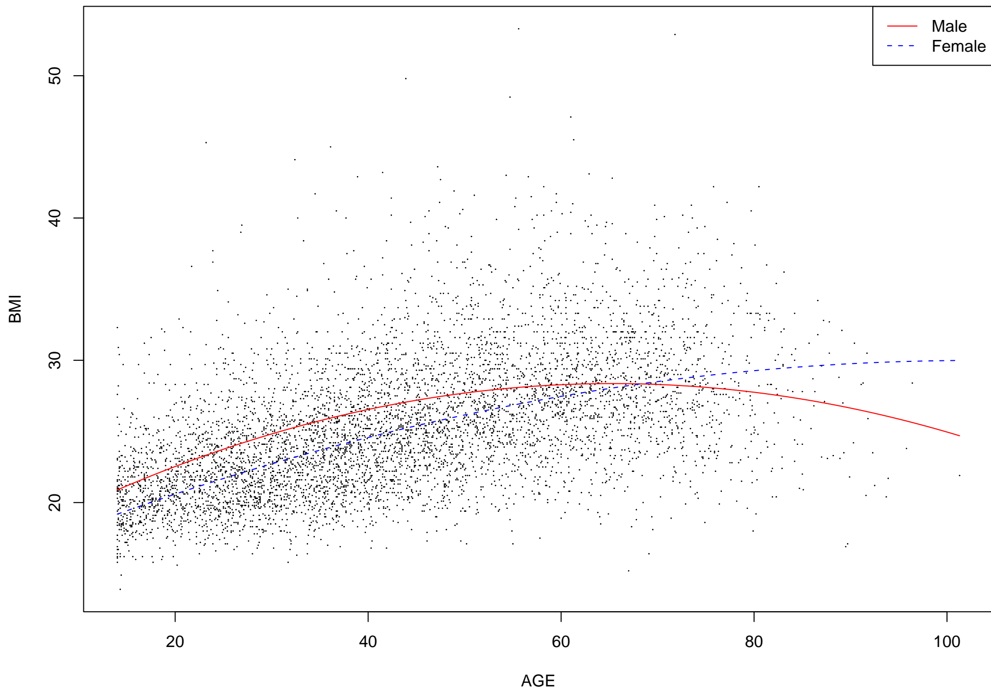
BMI plot against age
