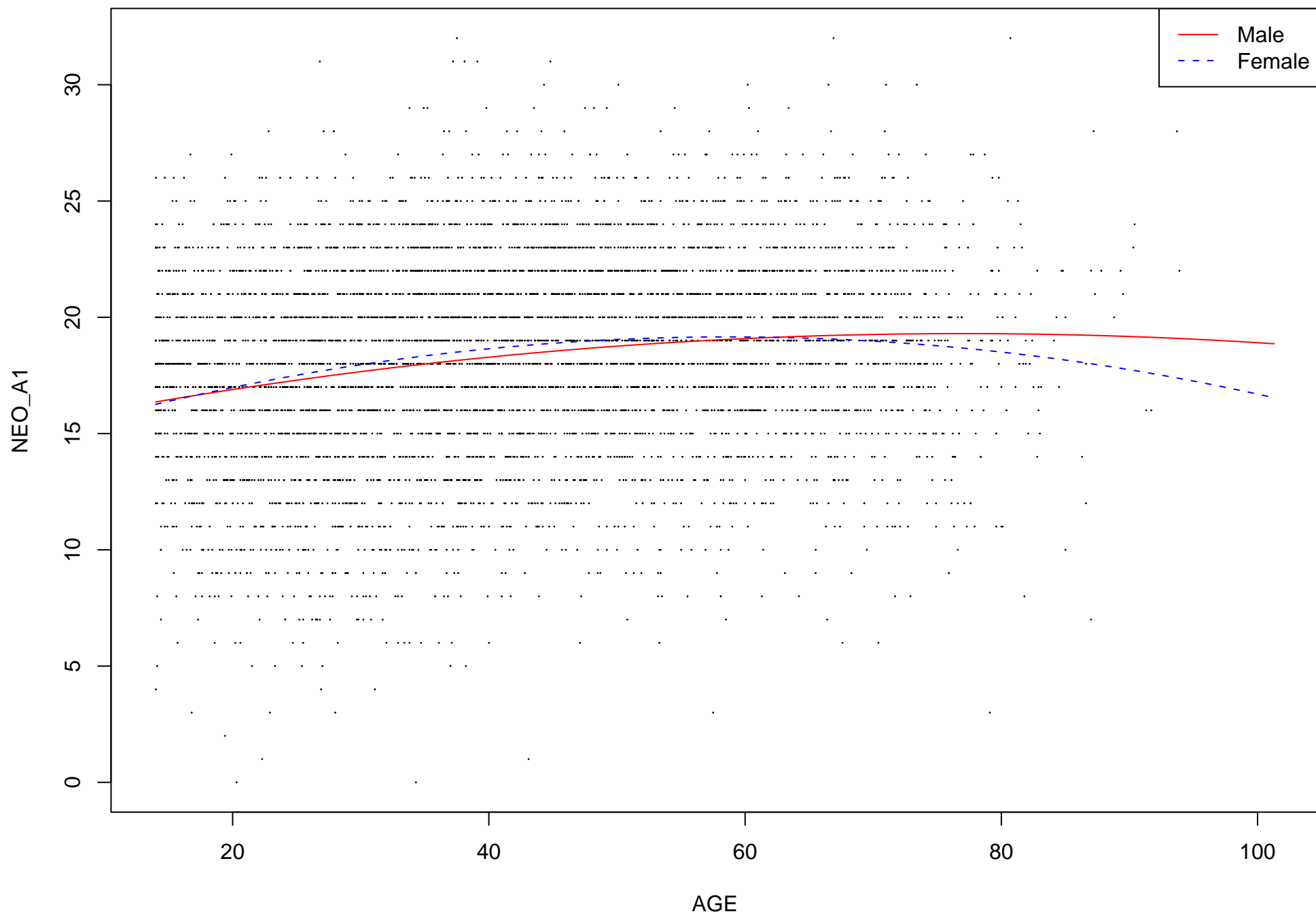
NEO_A1 plot against age
