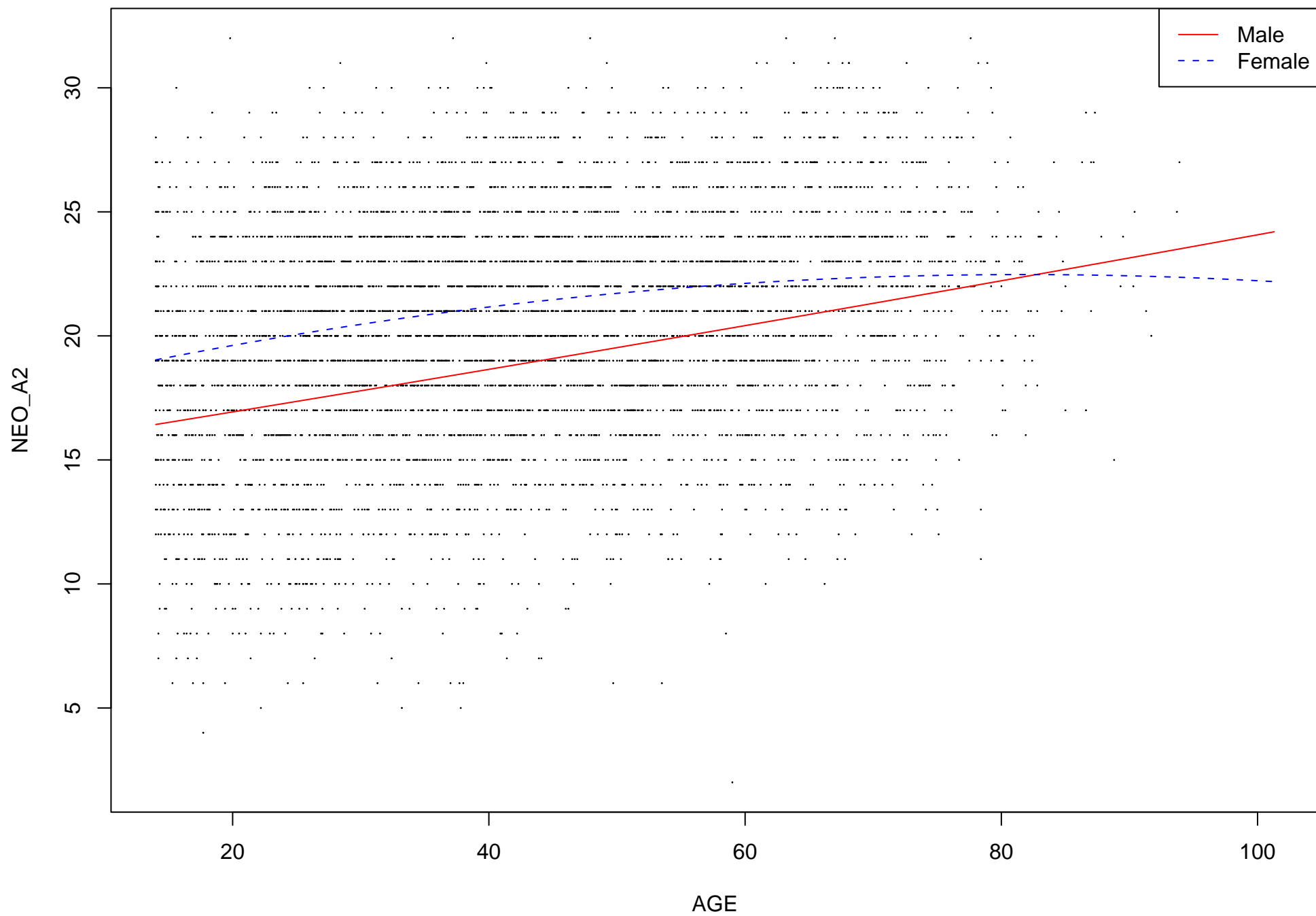
NEO_A2 plot against age
