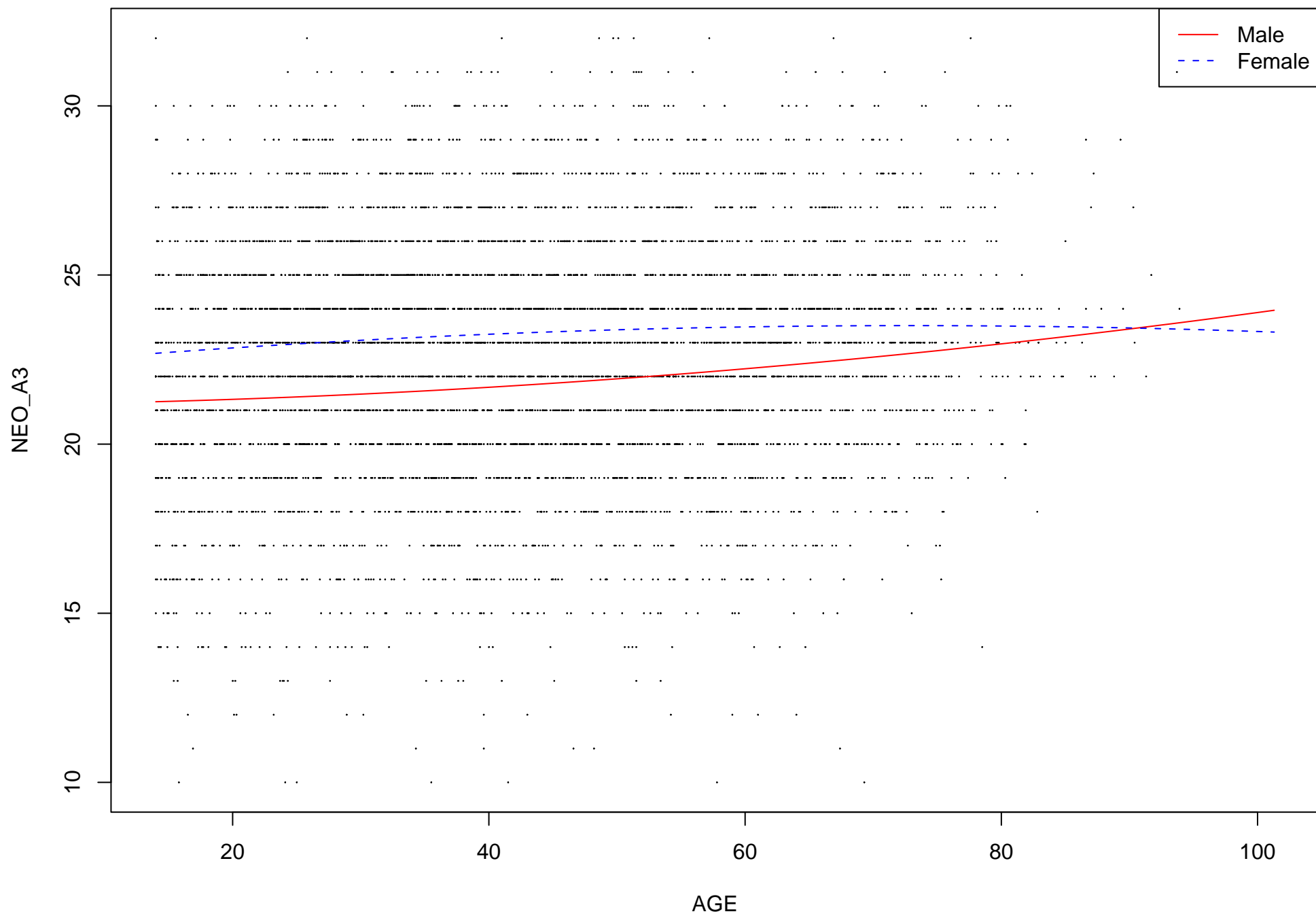
NEO_A3 plot against age
