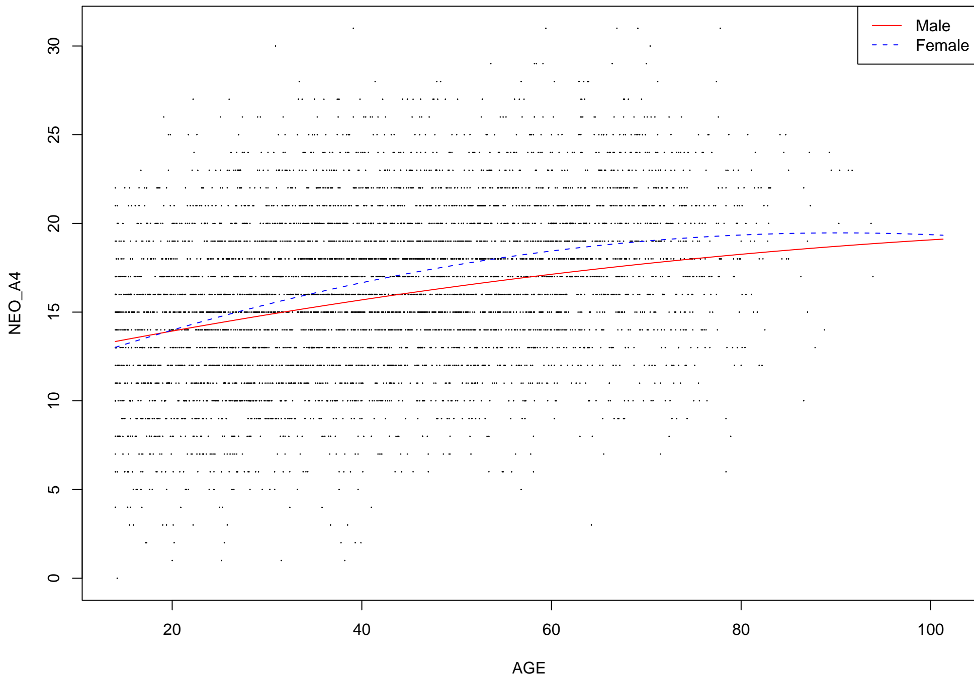
NEO_A4 plot against age
