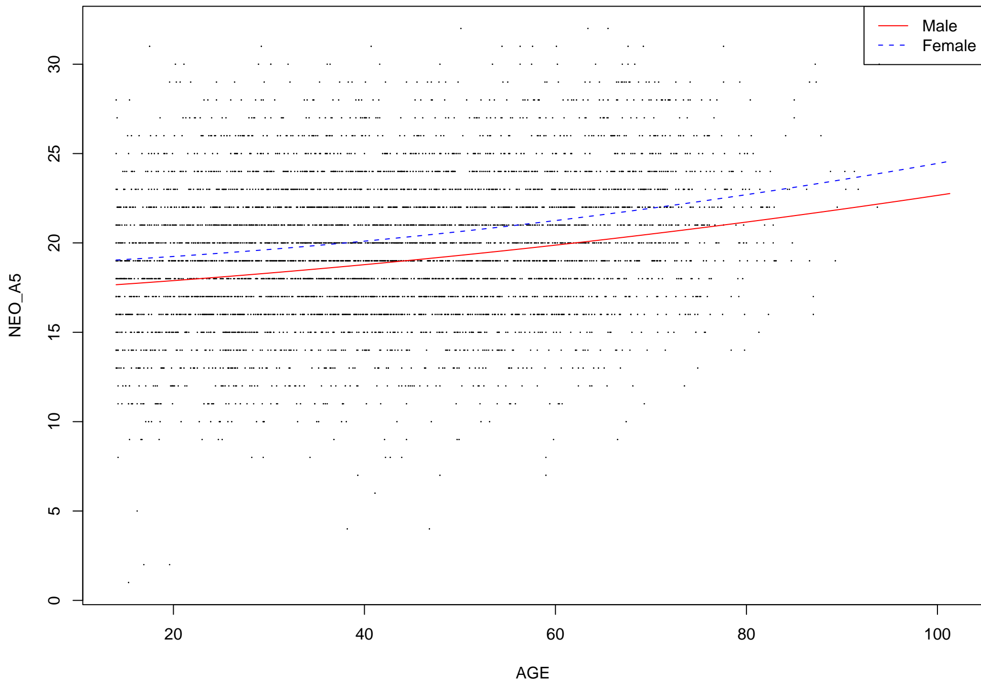
NEO_A5 plot against age
