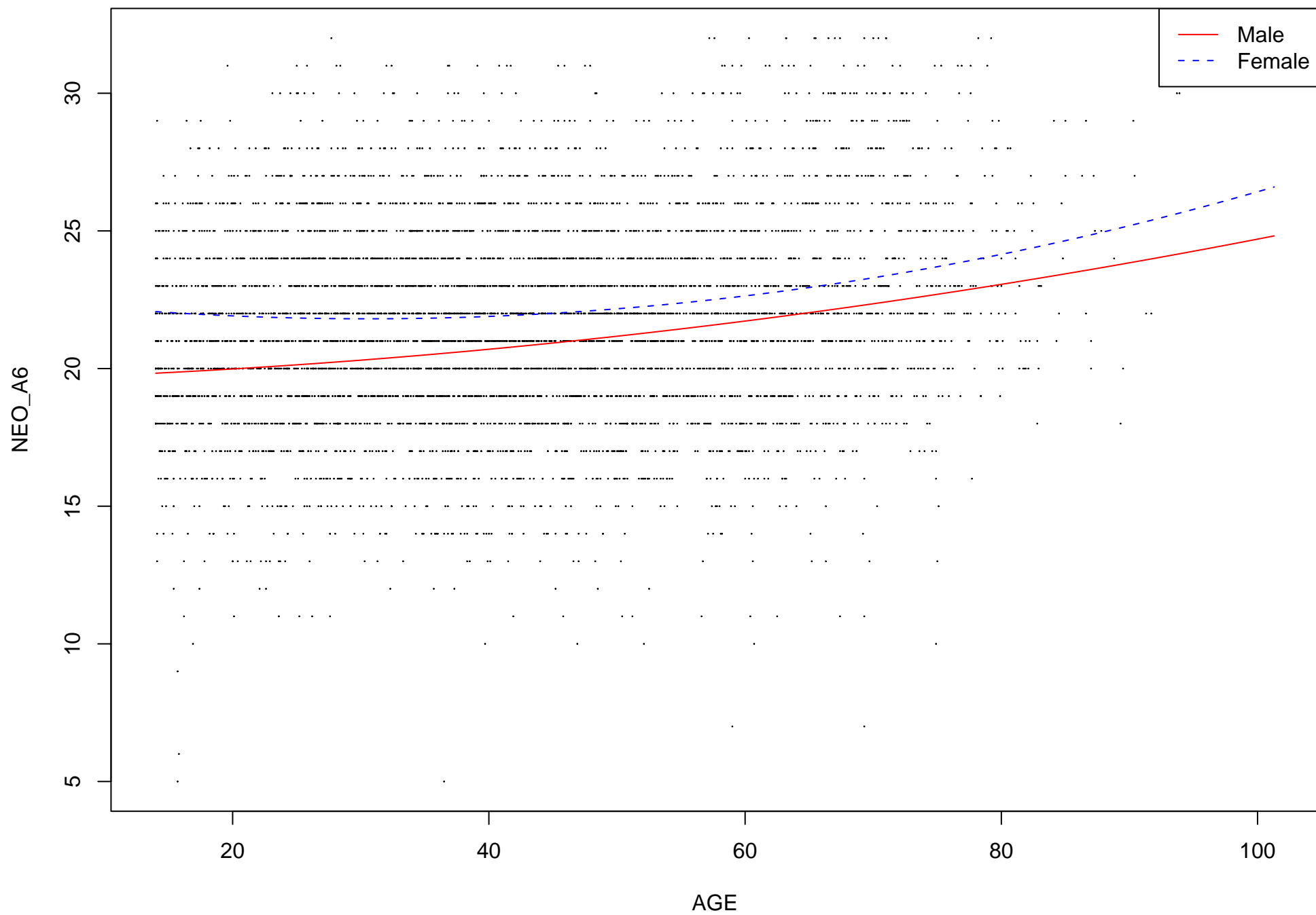
NEO_A6 plot against age
