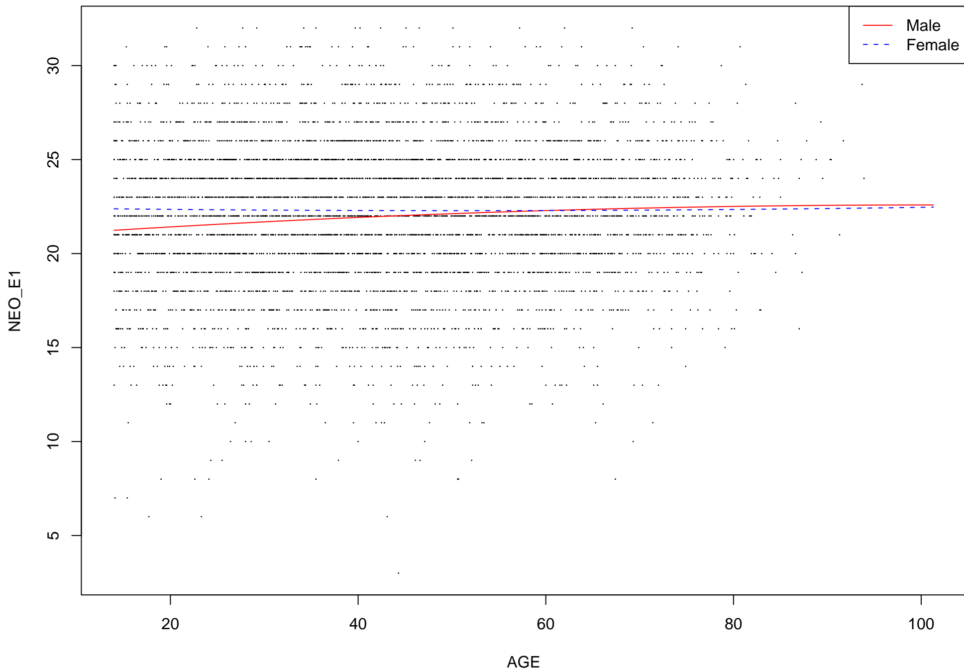
NEO_E1 plot against age
