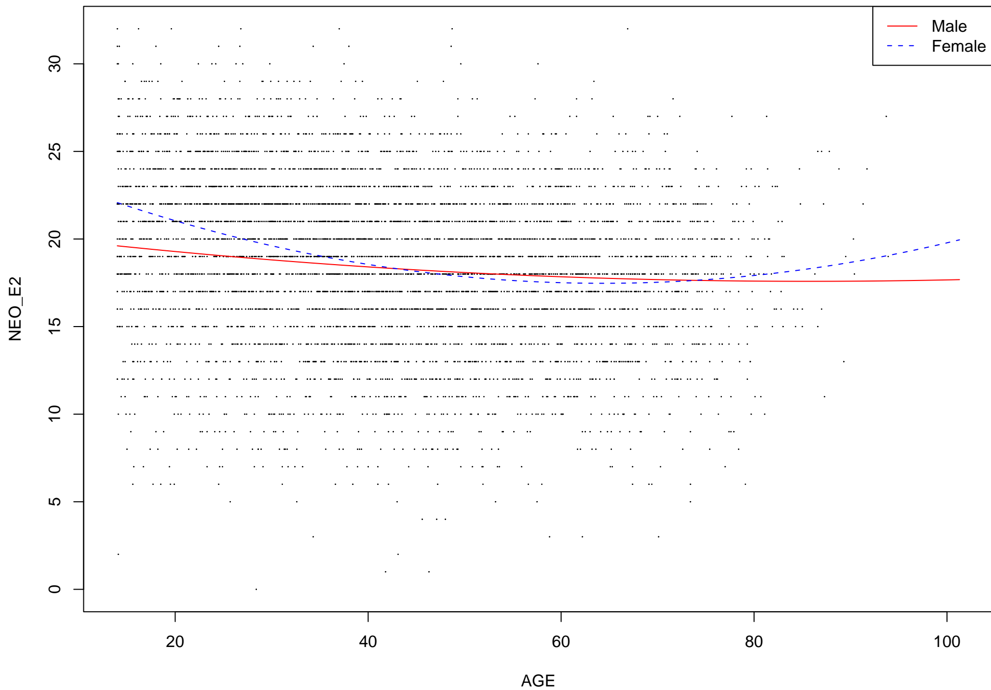
NEO_E2 plot against age
