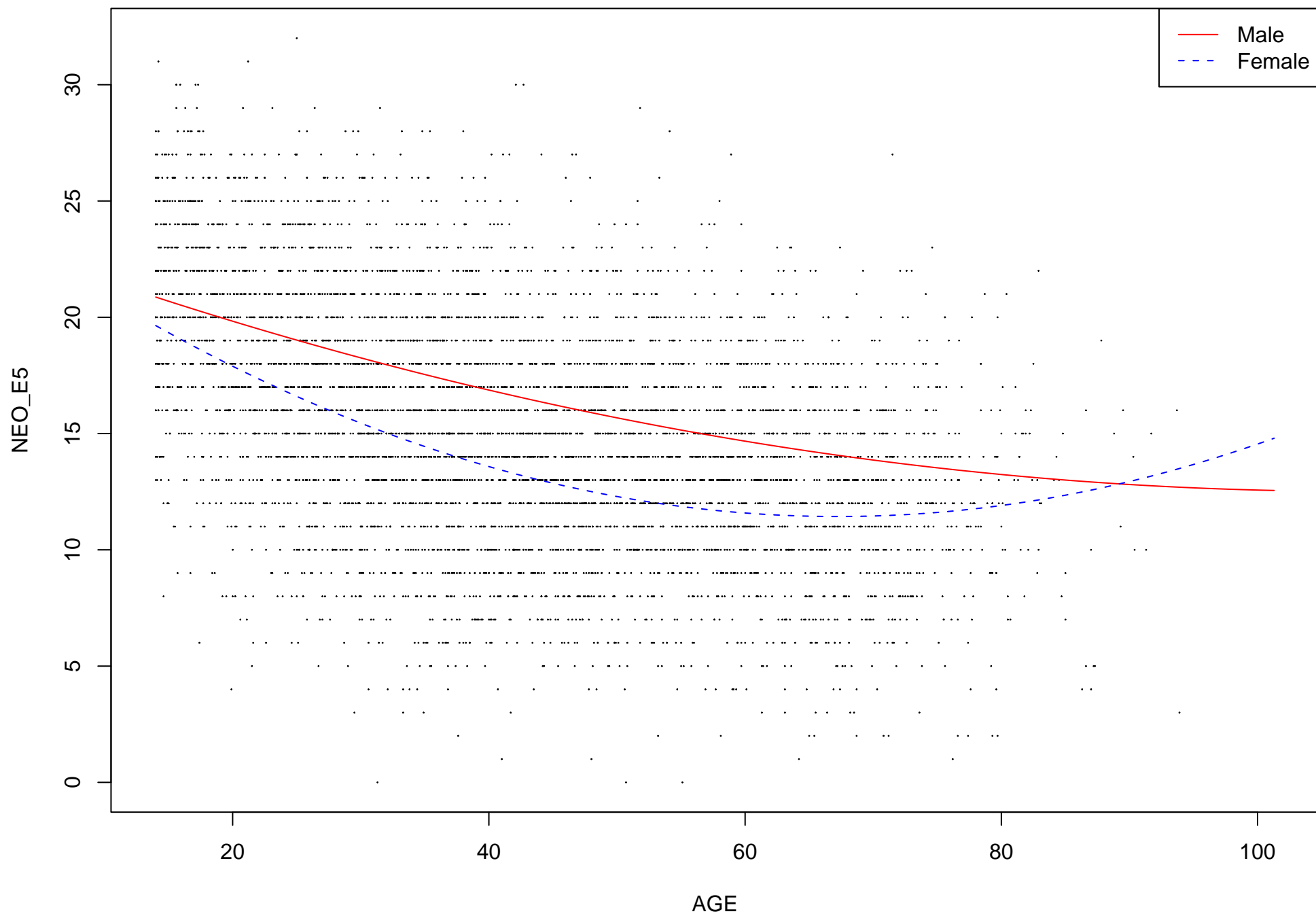
NEO_E5 plot against age
