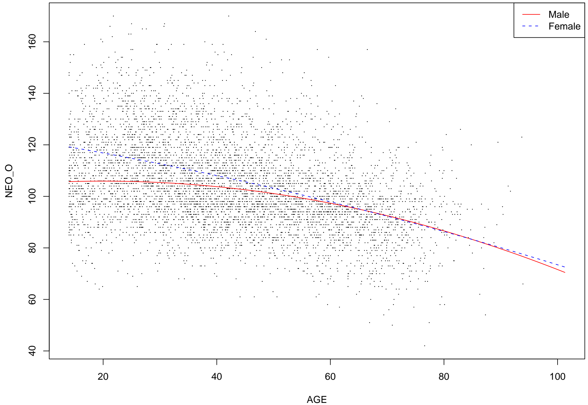
NEO_O plot against age
