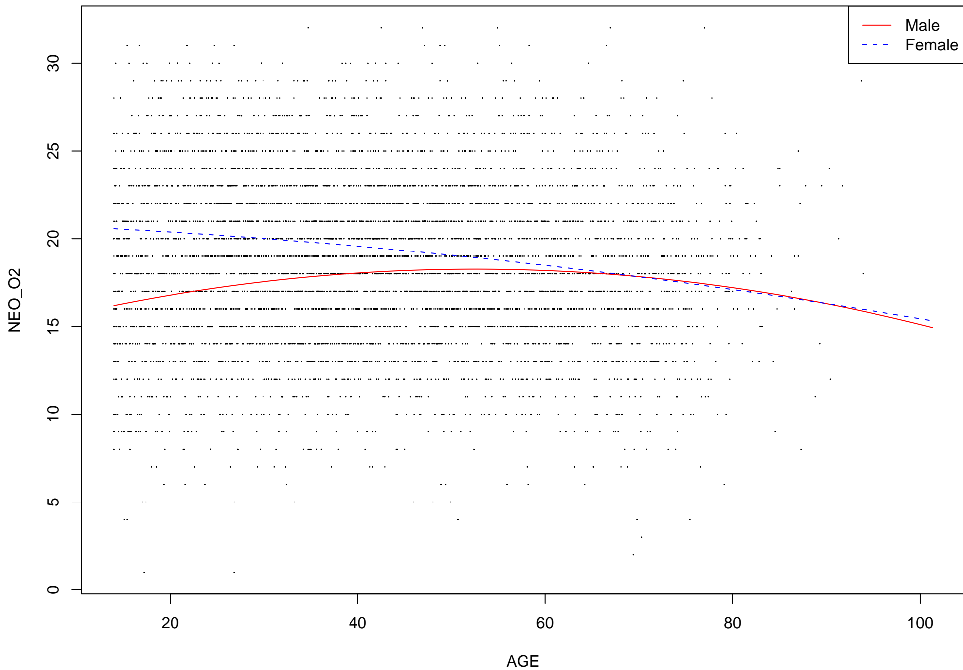
NEO_O2 plot against age
