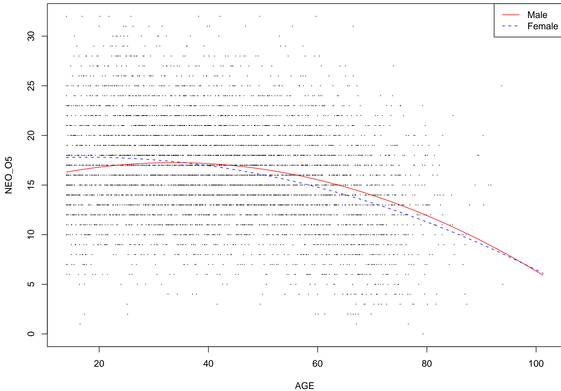
NEO_O5 plot against age
