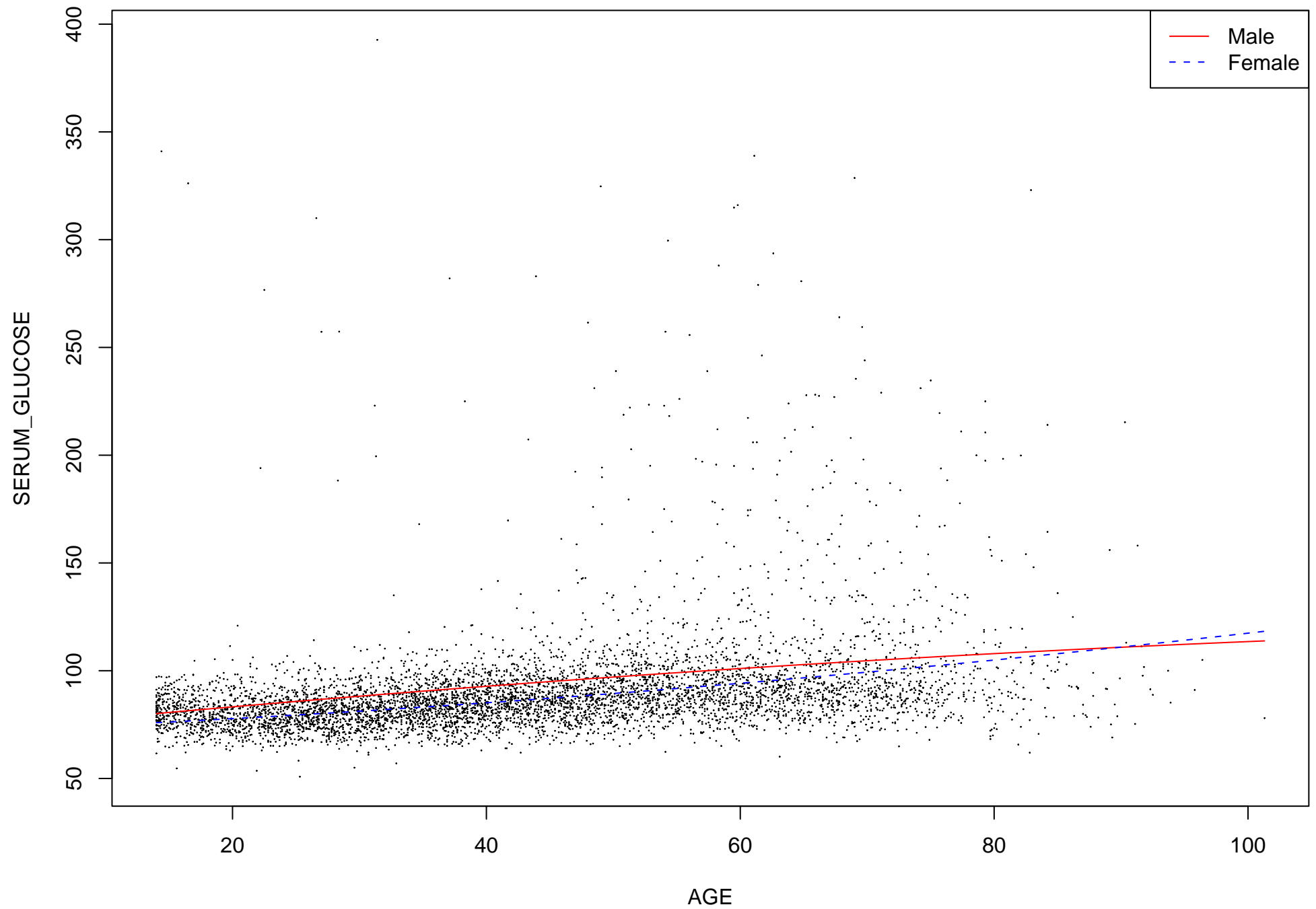
SERUM_GLUCOSE plot against age
