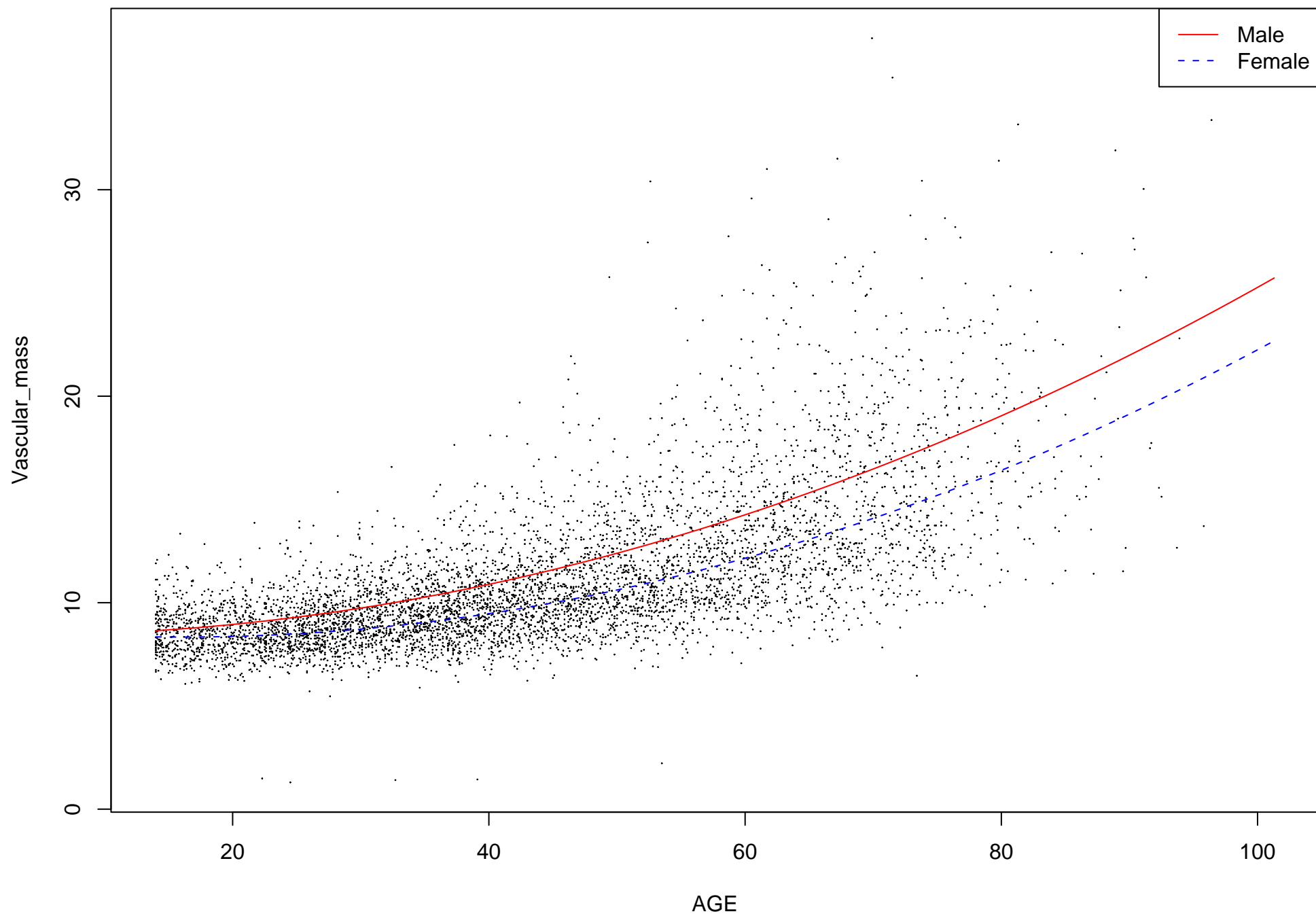
Vascular_mass plot against age
