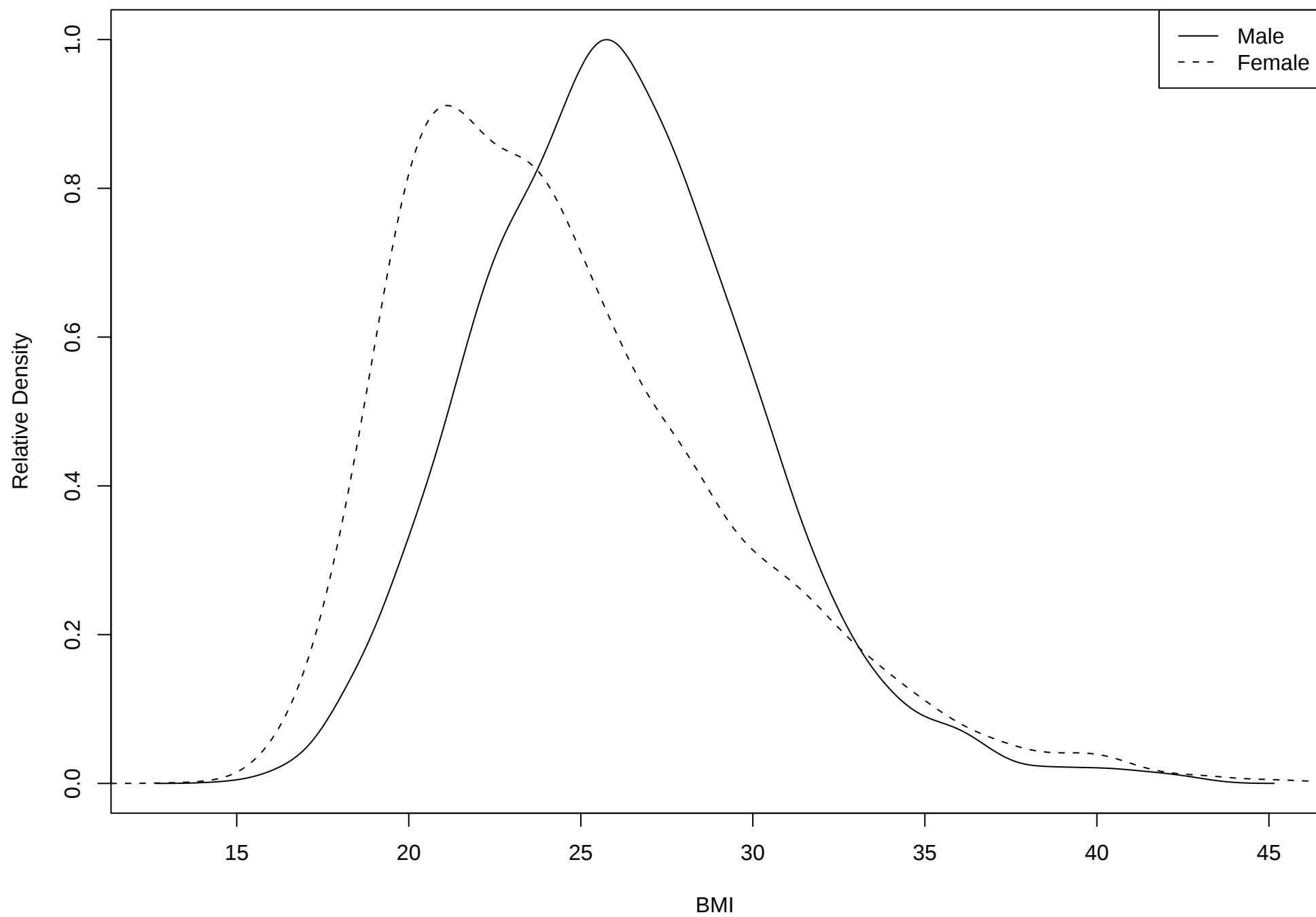
Density of trait BMI
