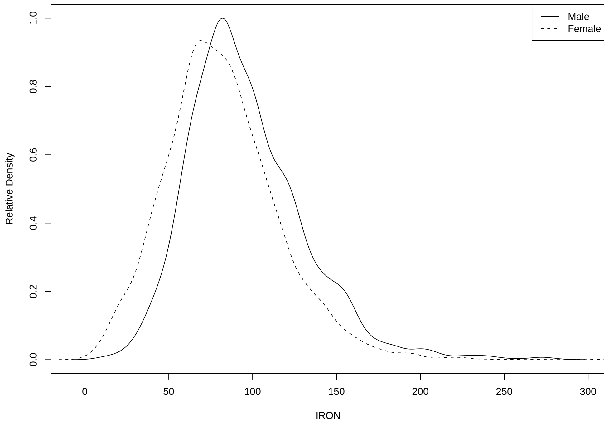
Density of trait IRON
