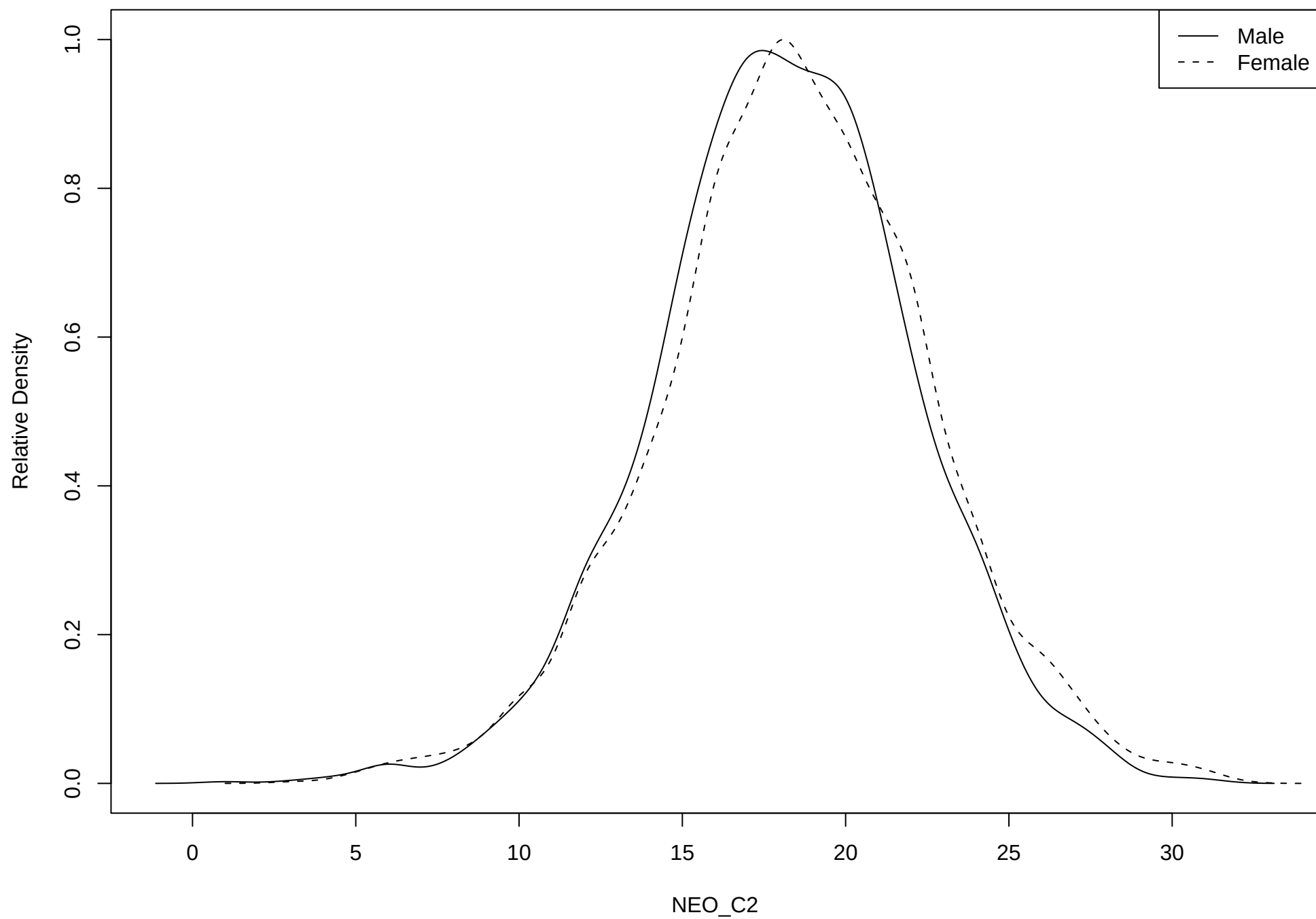
Density of trait NEO_C2
