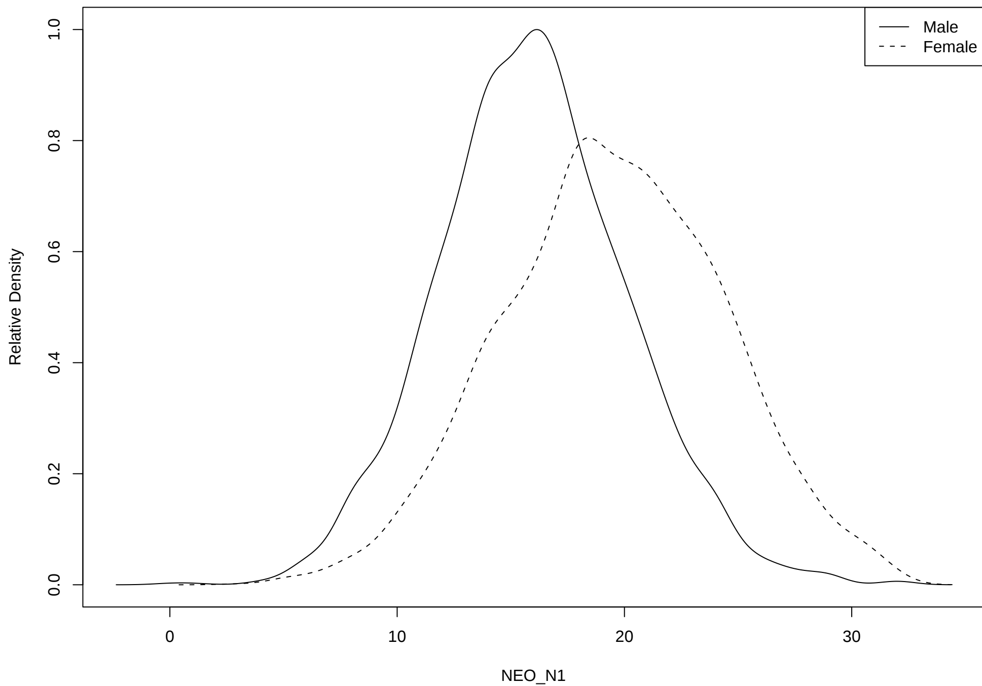
Density of trait NEO_N1
