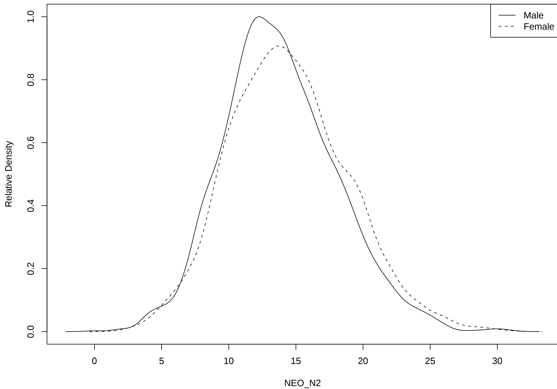
Density of trait NEO_N2
