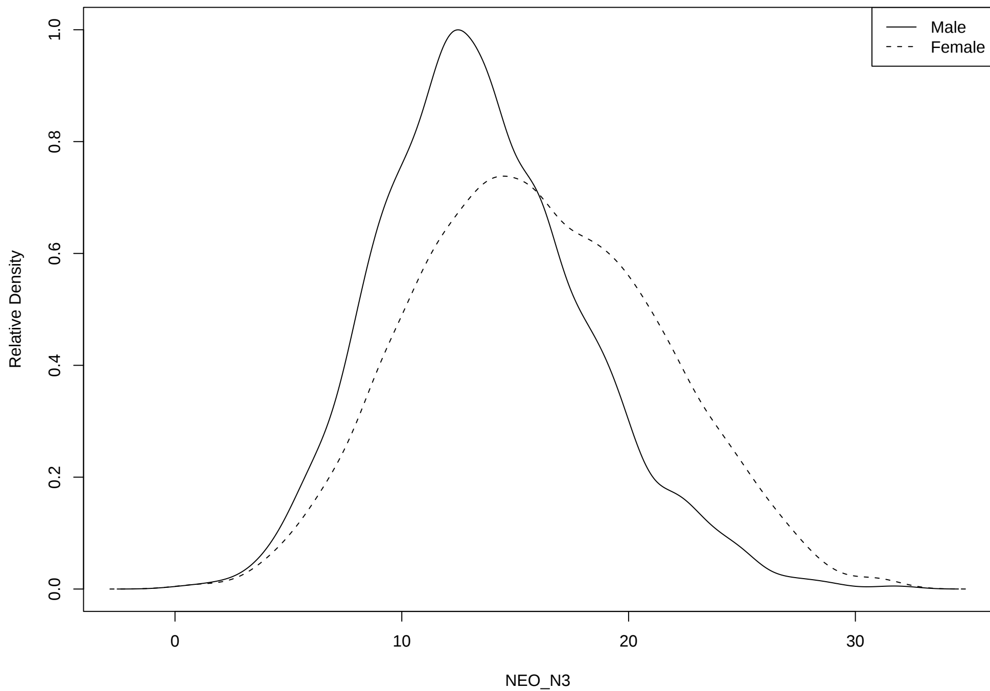
Density of trait NEO_N3
