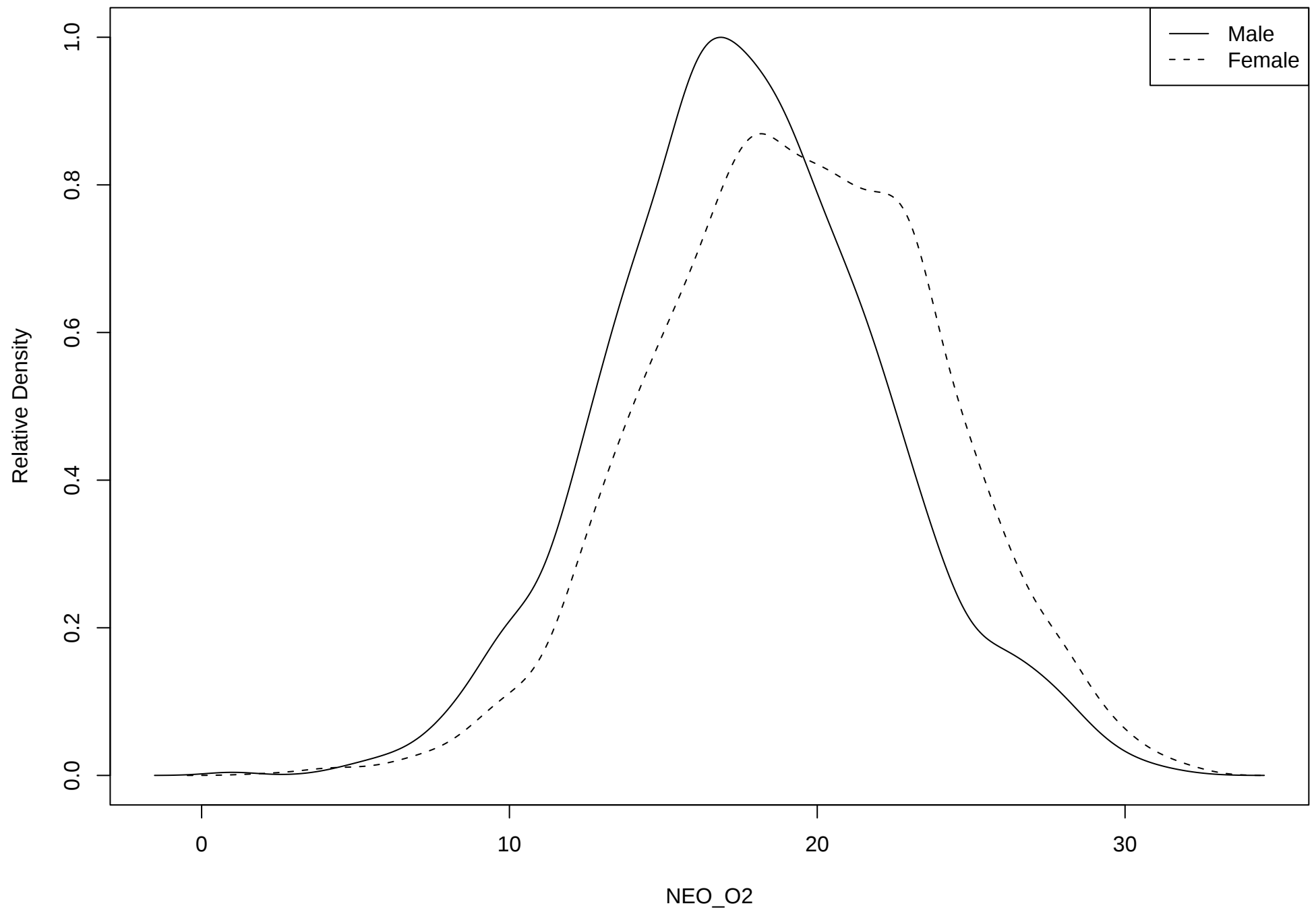
Density of trait NEO_O2
