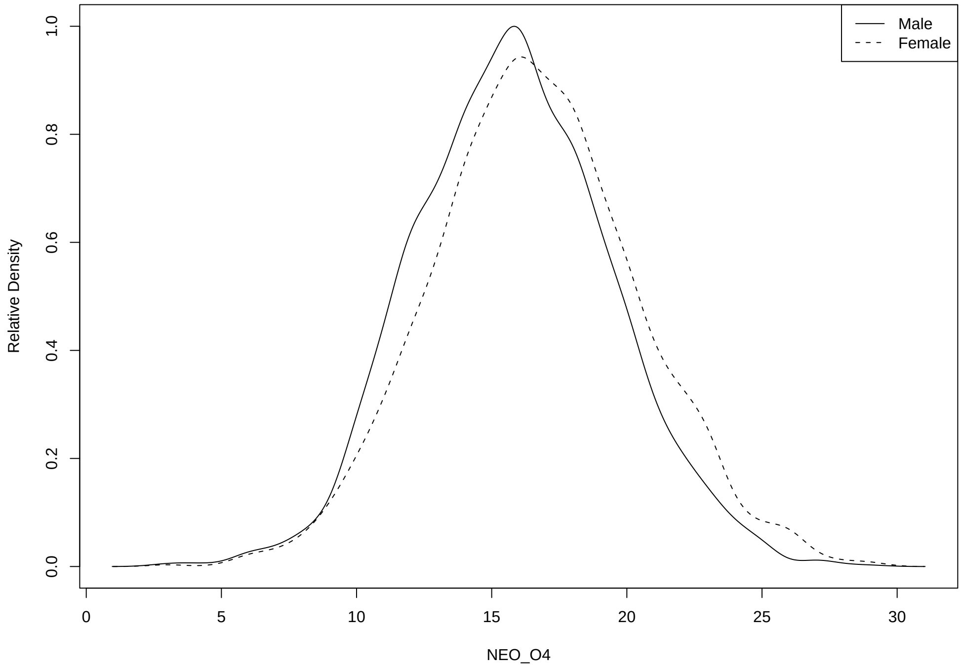
Density of trait NEO_O4
