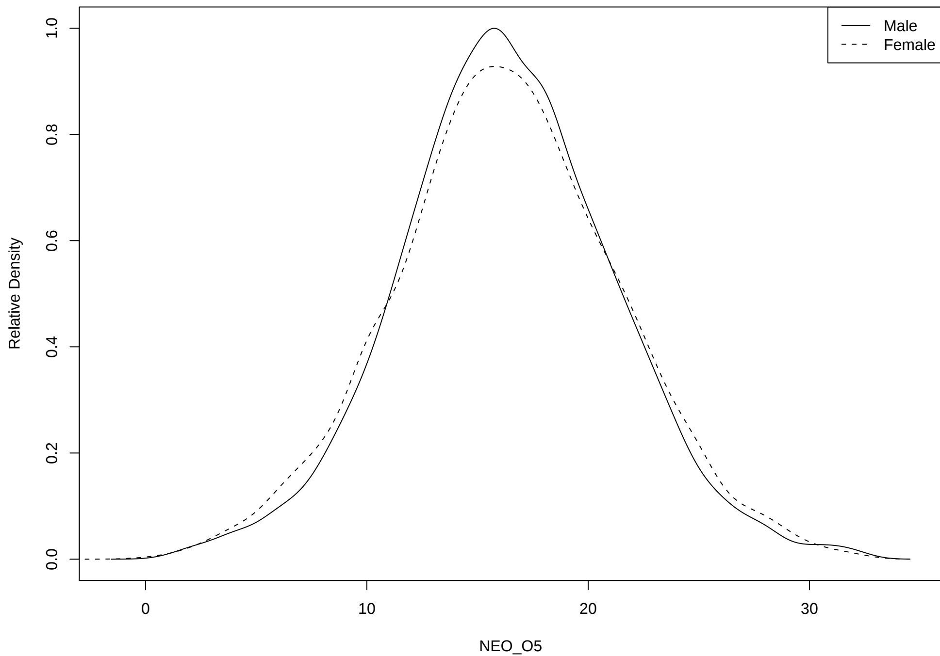
Density of trait NEO_O5
