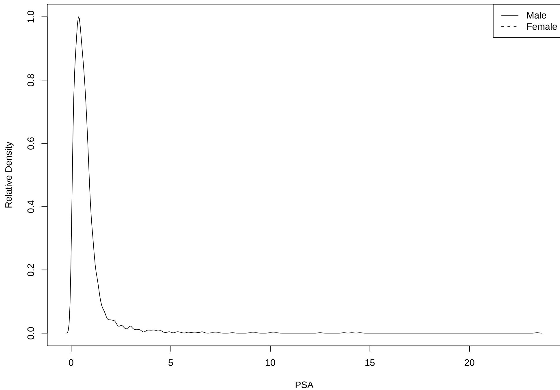
Density of trait PSA
