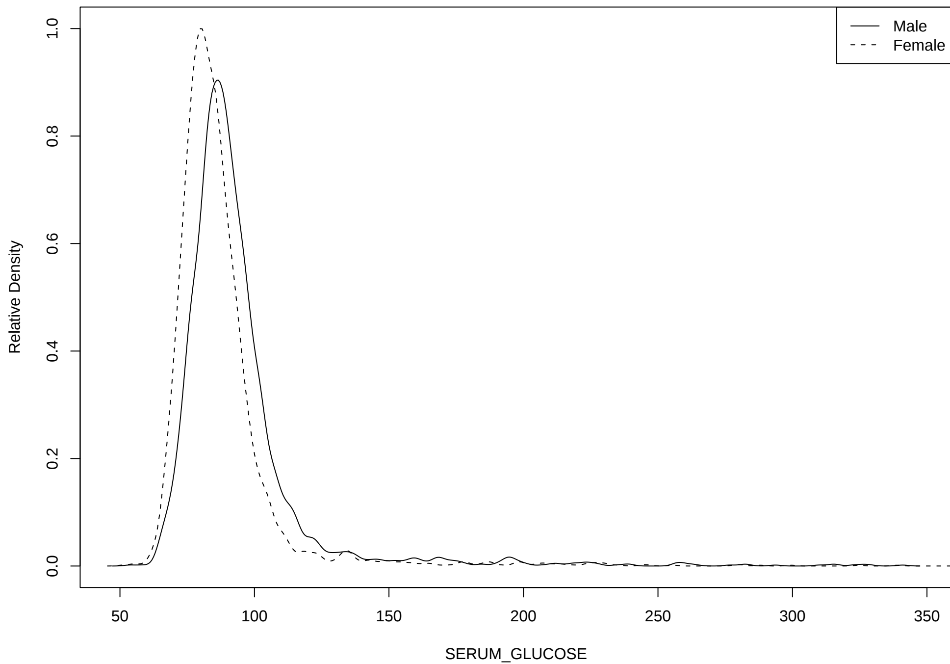
Density of trait SERUM_GLUCOSE
