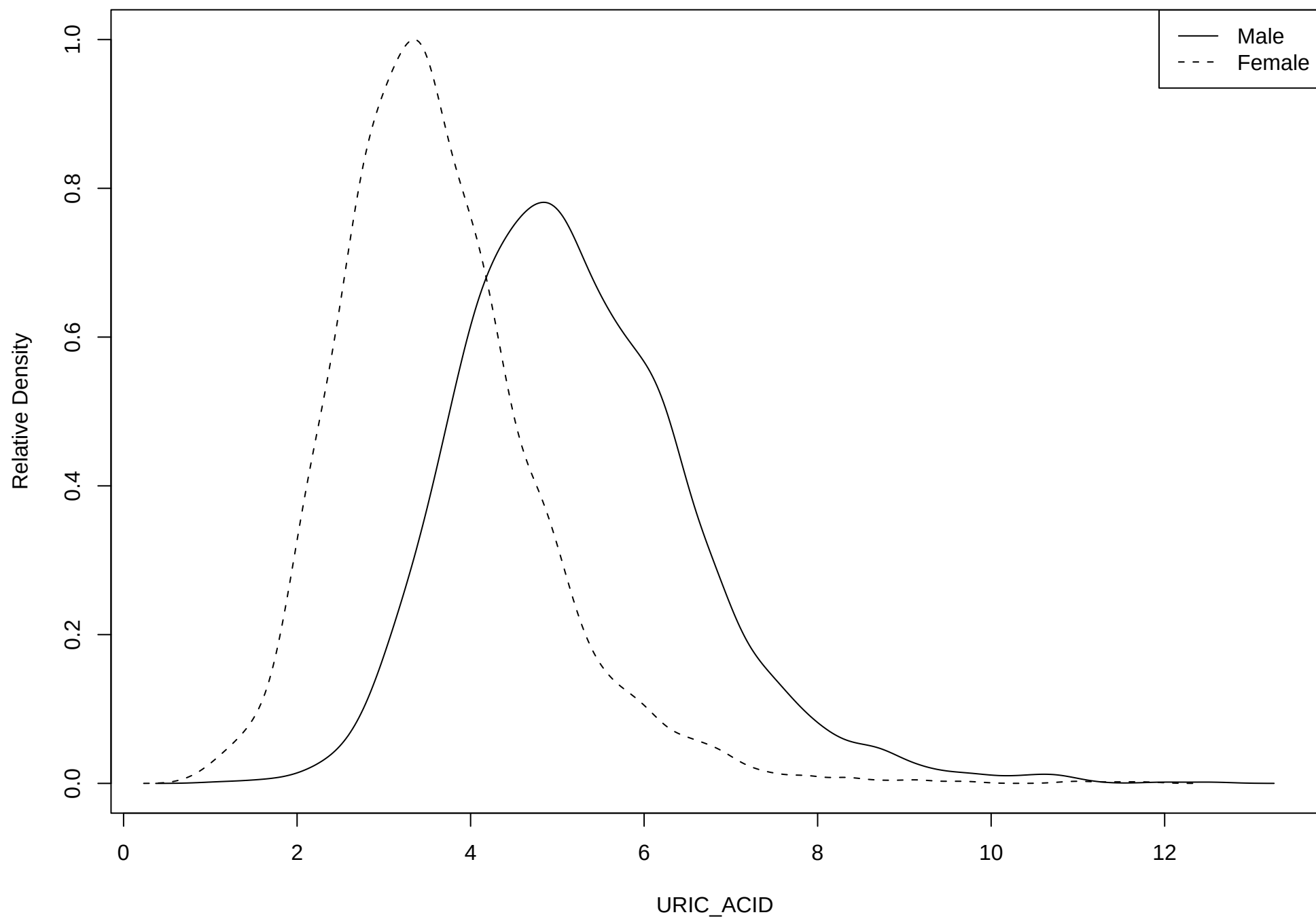
Density of trait URIC_ACID
