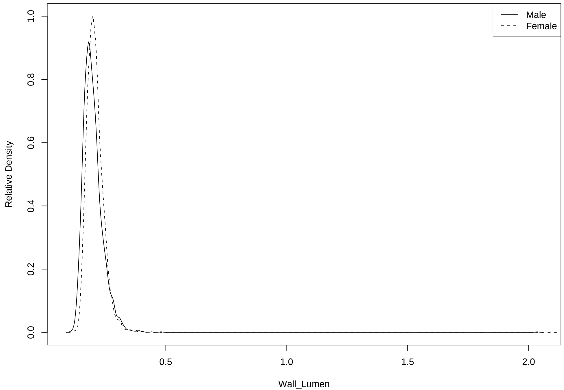
Density of trait Wall_Lumen
