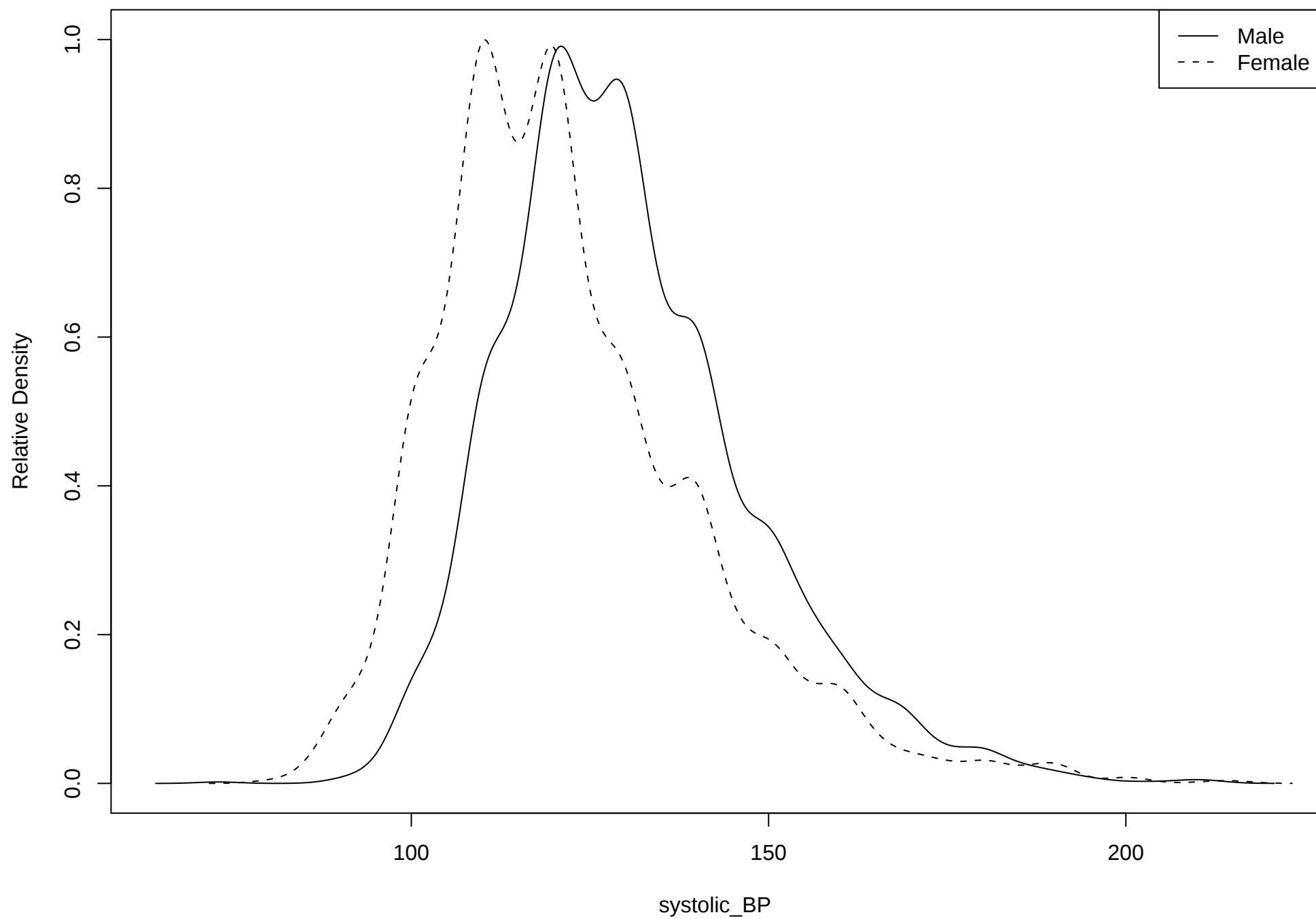
Density of trait systolic_BP
