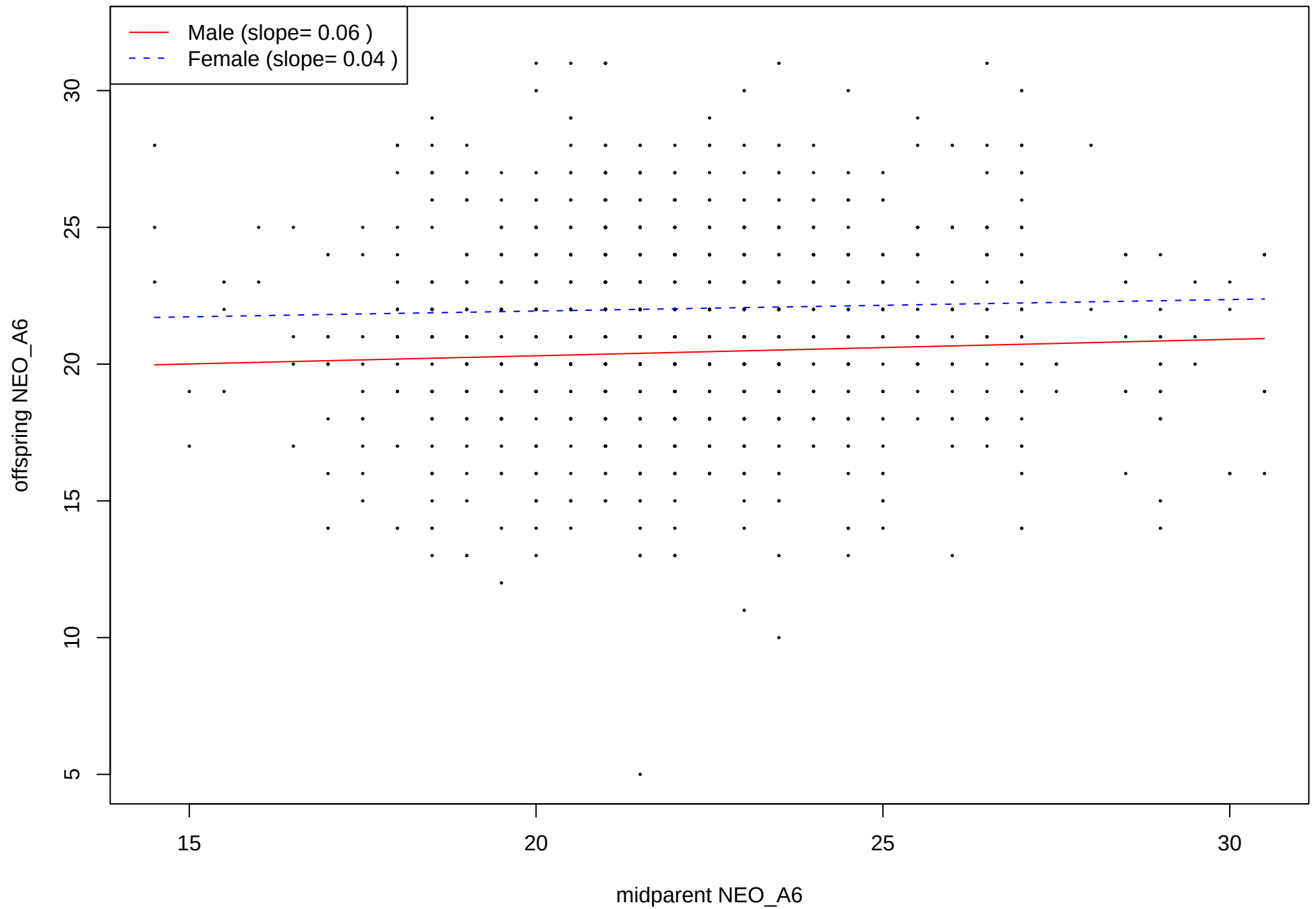
Regression of midparent NEO_A6 on offspring
