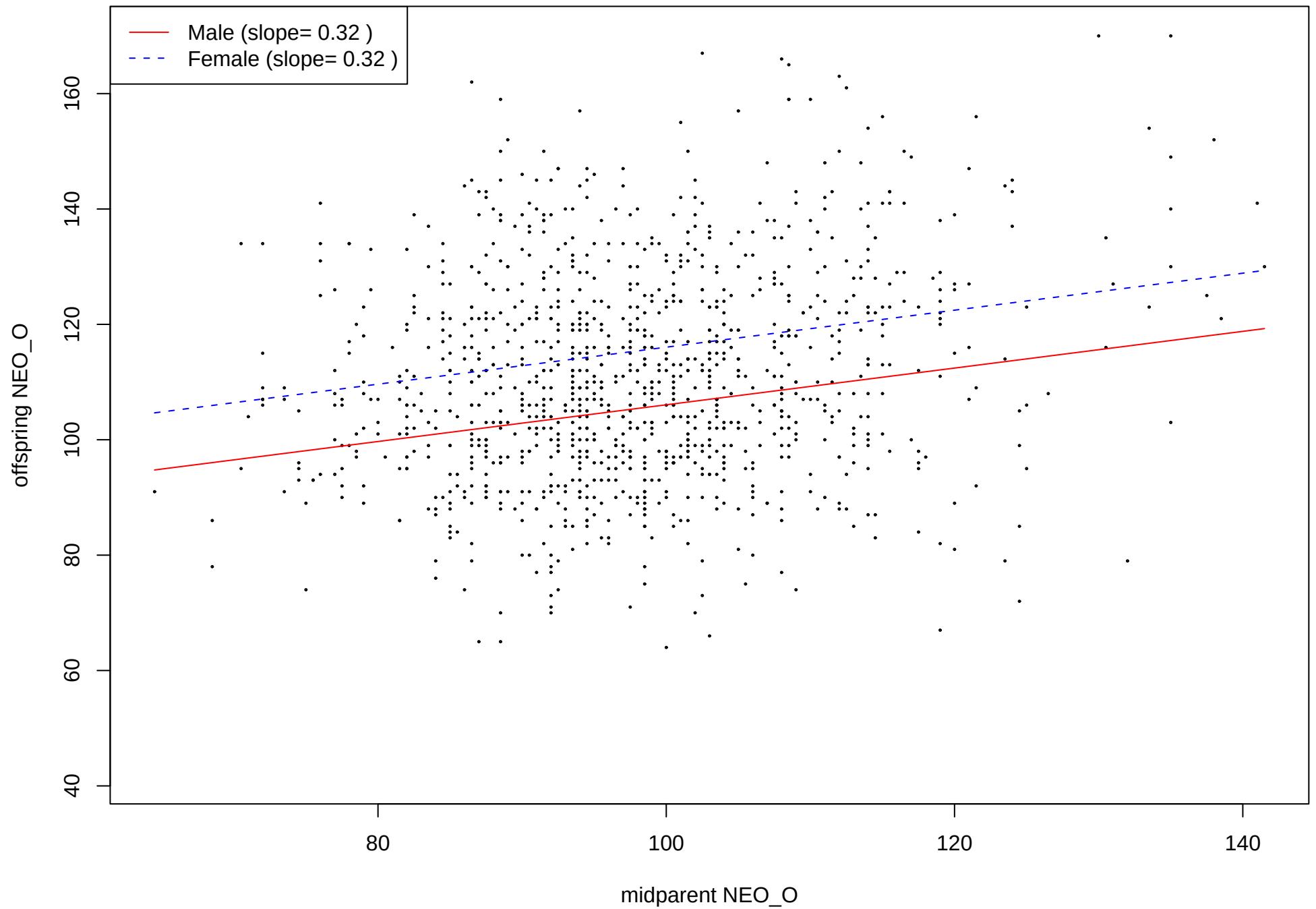
Regression of midparent NEO_O on offspring
