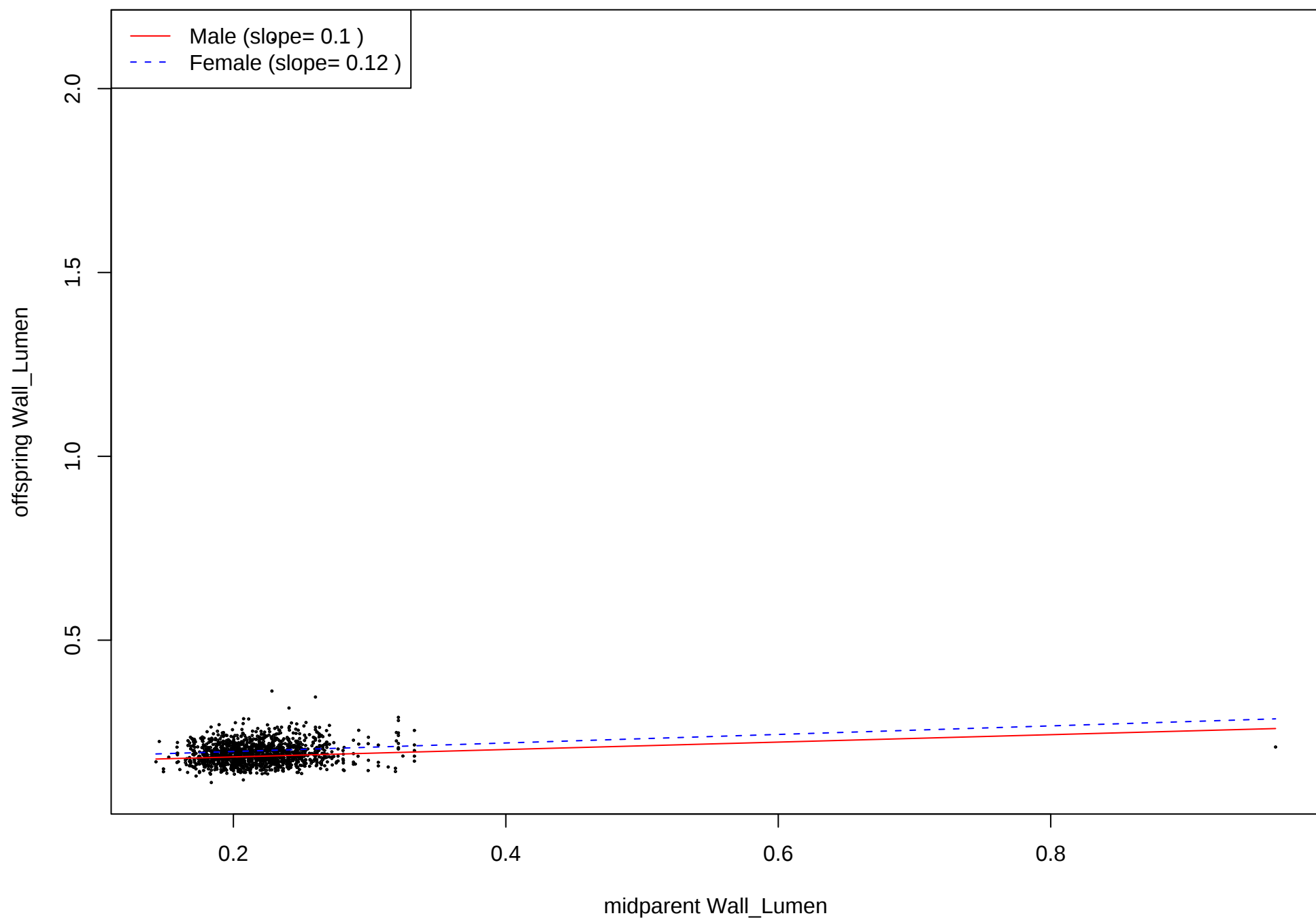
Regression of midparent Wall_Lumen on offspring
